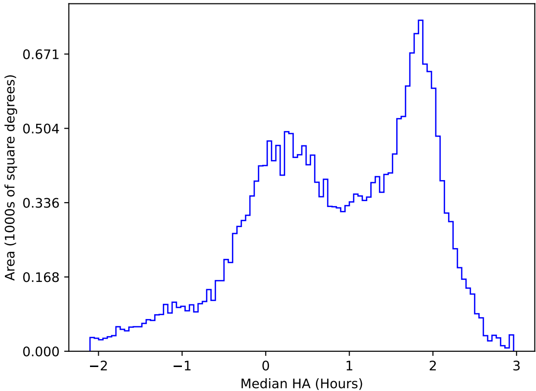
too_elab_r256_d2_ugrizy_v3.4_10yrs All sky u band: Median HA
