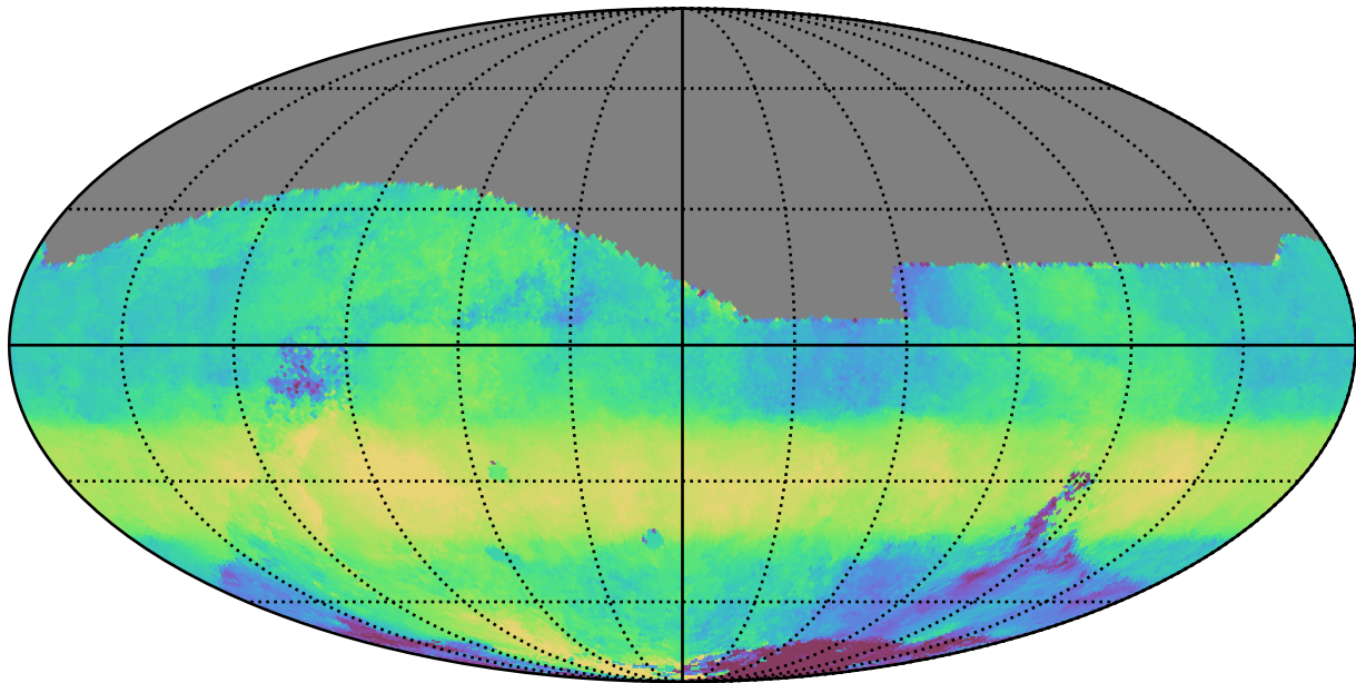
too_elab_r256_d2_ugrizy_v3.4_10yrs All sky r band: Median HA
