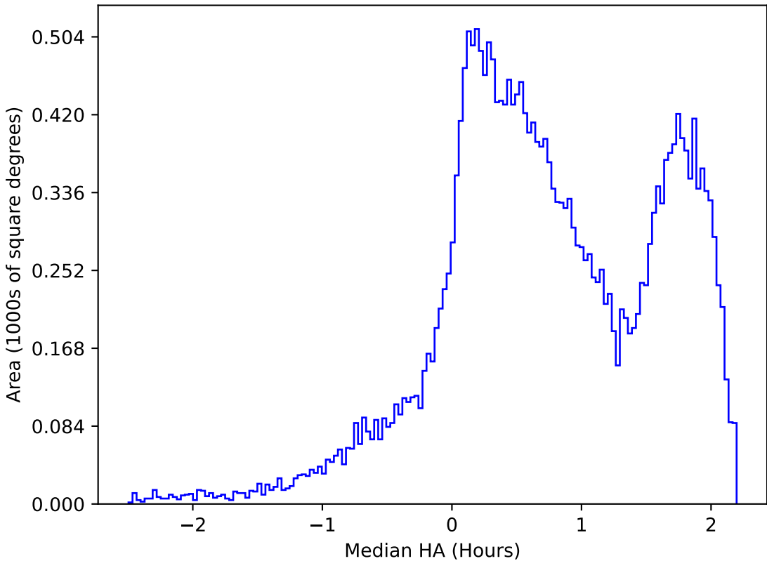
too_elab_r256_d2_ugrizy_v3.4_10yrs All sky r band: Median HA
