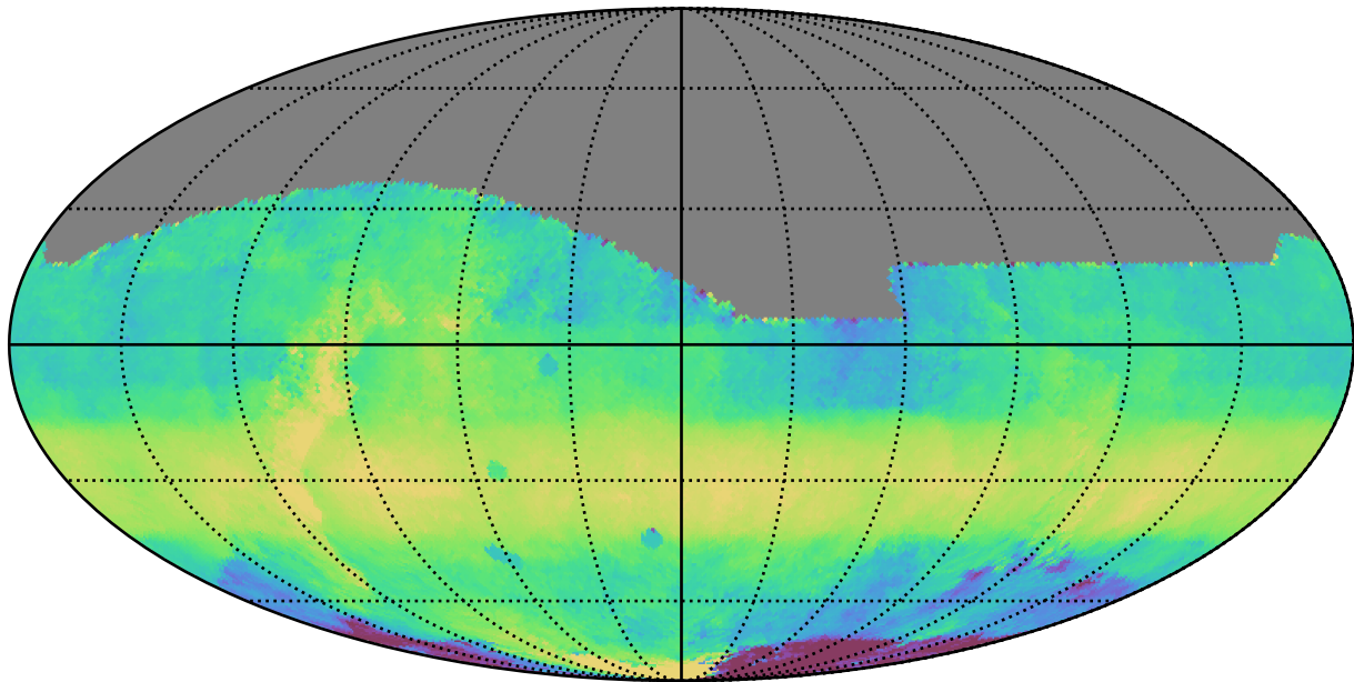
too_elab_r256_d2_ugrizy_v3.4_10yrs All sky i band: Median HA
