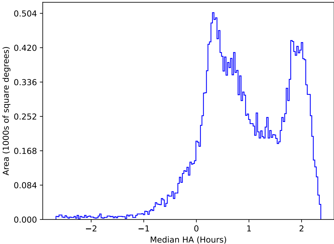
too_elab_r256_d2_ugrizy_v3.4_10yrs All sky i band: Median HA
