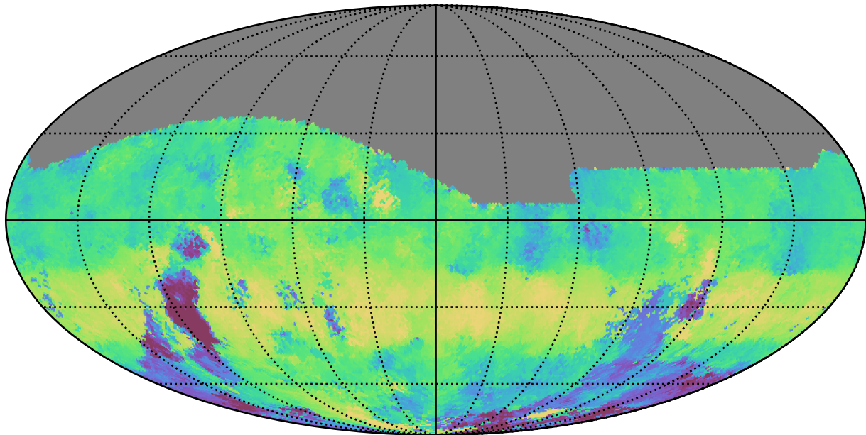
too_elab_r256_d2_ugrizy_v3.4_10yrs All sky g band: Median HA
