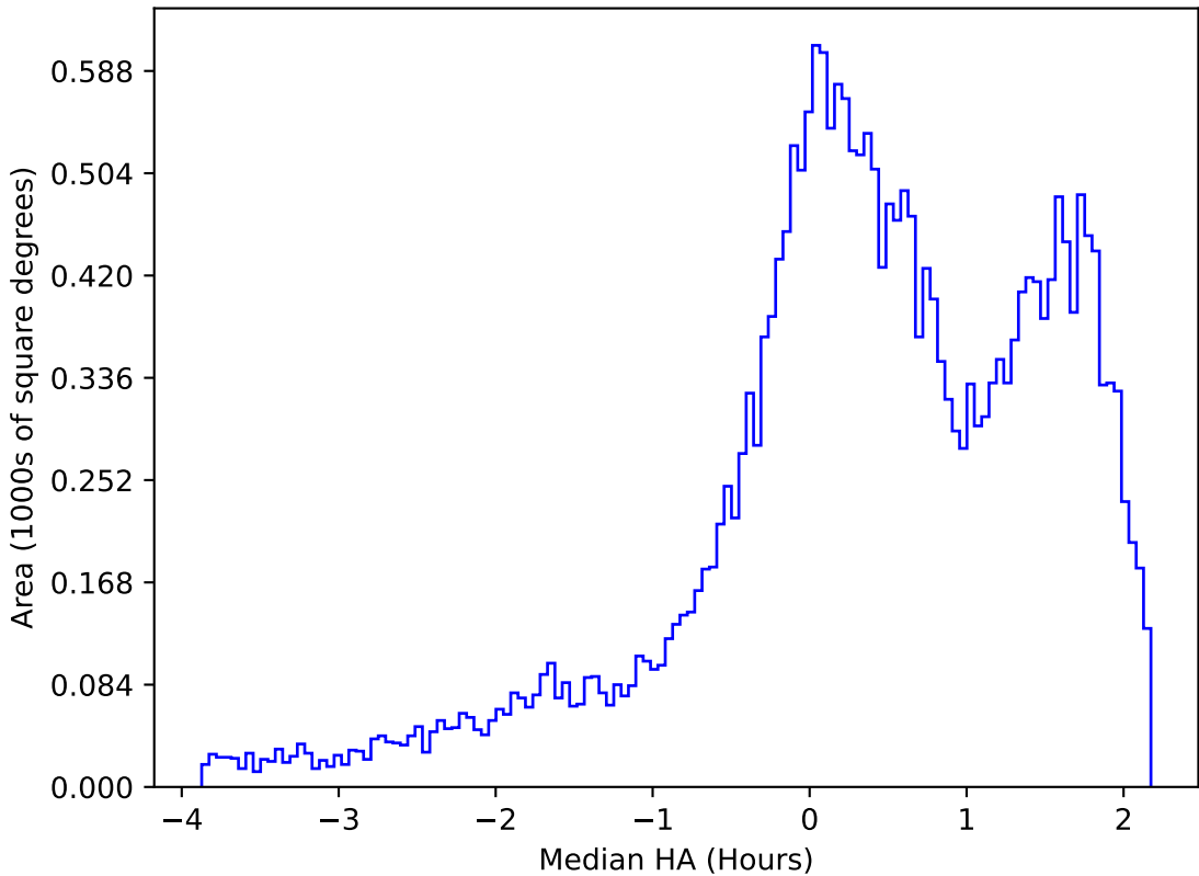
too_elab_r256_d2_ugrizy_v3.4_10yrs All sky g band: Median HA
