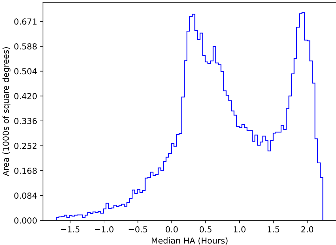
too_elab_r256_d2_ugrizy_v3.4_10yrs All sky all bands: Median HA
