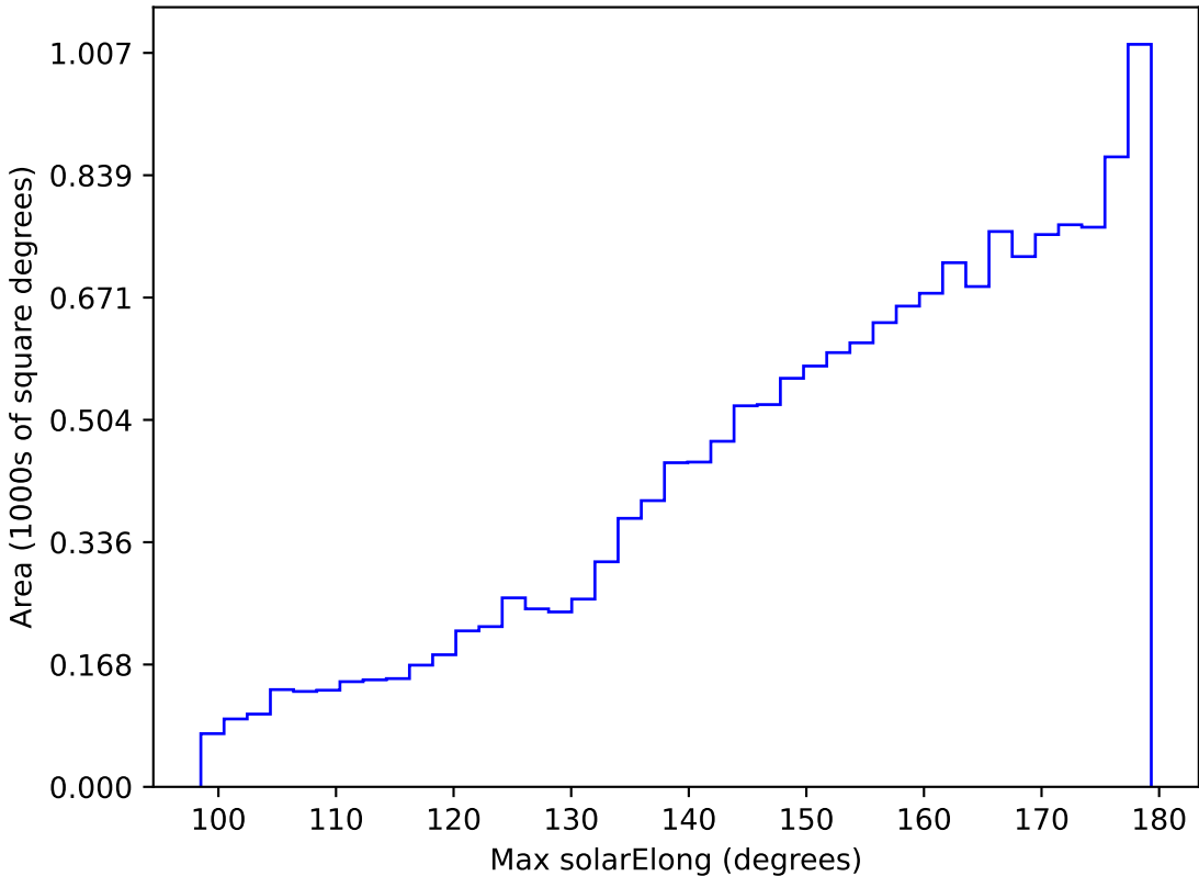
too_elab_r256_d2_ugrizy_v3.4_10yrs WFD z band: Max solarElong
