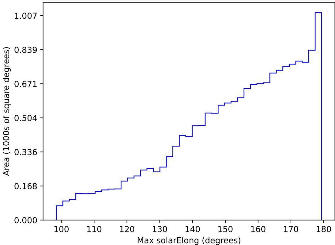
too_elab_r256_d2_ugrizy_v3.4_10yrs WFD r band: Max solarElong
