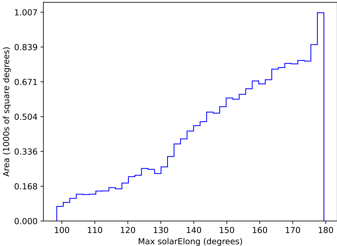
too_elab_r256_d2_ugrizy_v3.4_10yrs WFD i band: Max solarElong
