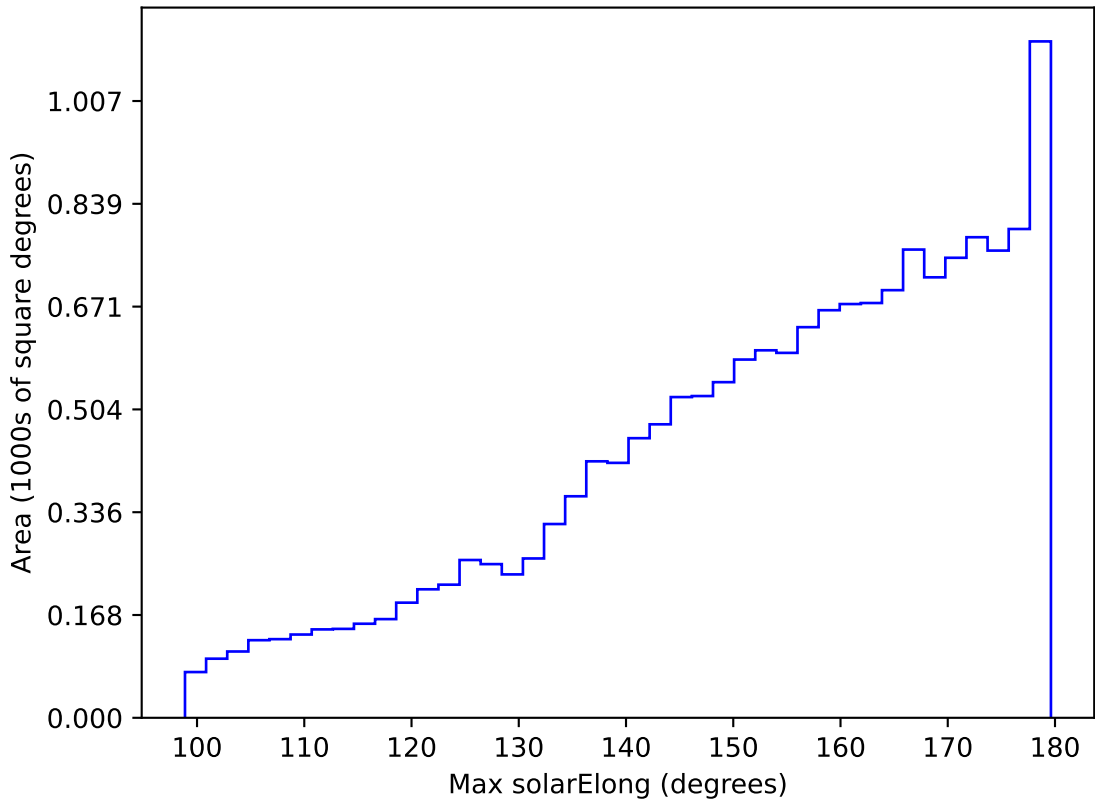
too_elab_r256_d2_ugrizy_v3.4_10yrs WFD all bands: Max solarElong
