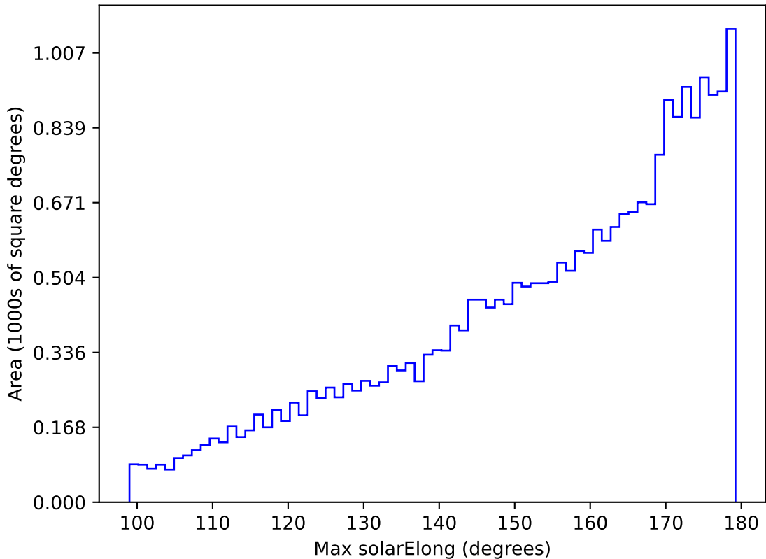
too_elab_r256_d2_ugrizy_v3.4_10yrs All sky z band: Max solarElong
