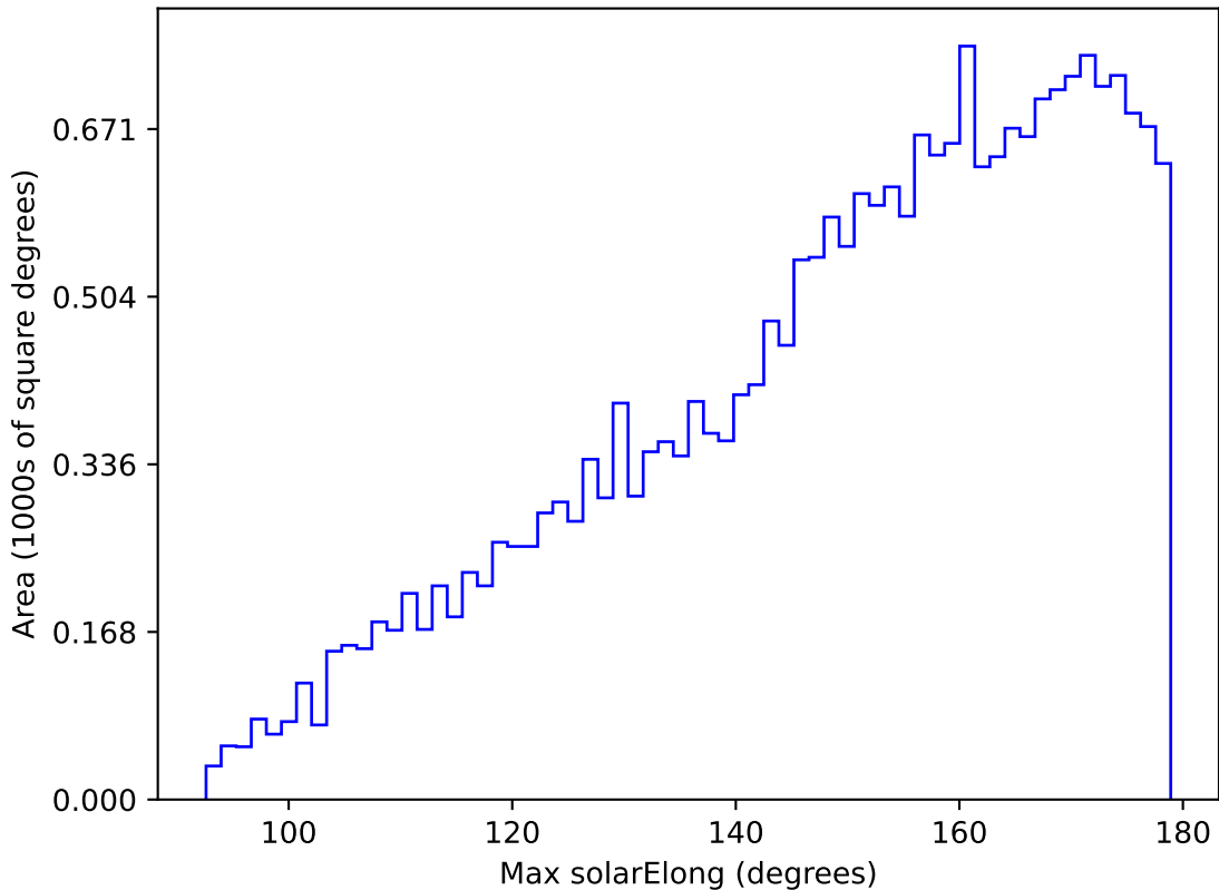
too_elab_r256_d2_ugrizy_v3.4_10yrs All sky u band: Max solarElong
