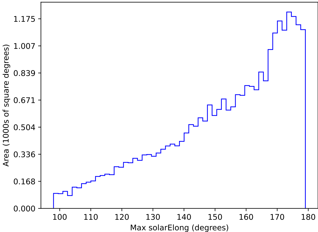
too_elab_r256_d2_ugrizy_v3.4_10yrs All sky g band: Max solarElong
