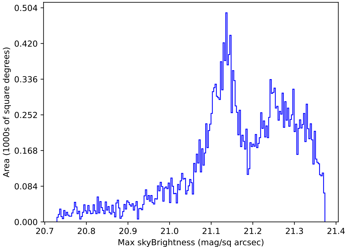
too_elab_r256_d2_ugrizy_v3.4_10yrs Yr 1 r band: Max skyBrightness
