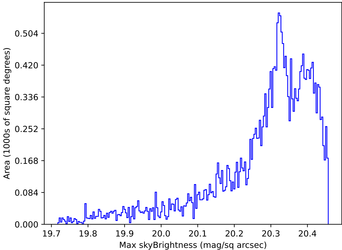
too_elab_r256_d2_ugrizy_v3.4_10yrs Yr 1 i band: Max skyBrightness
