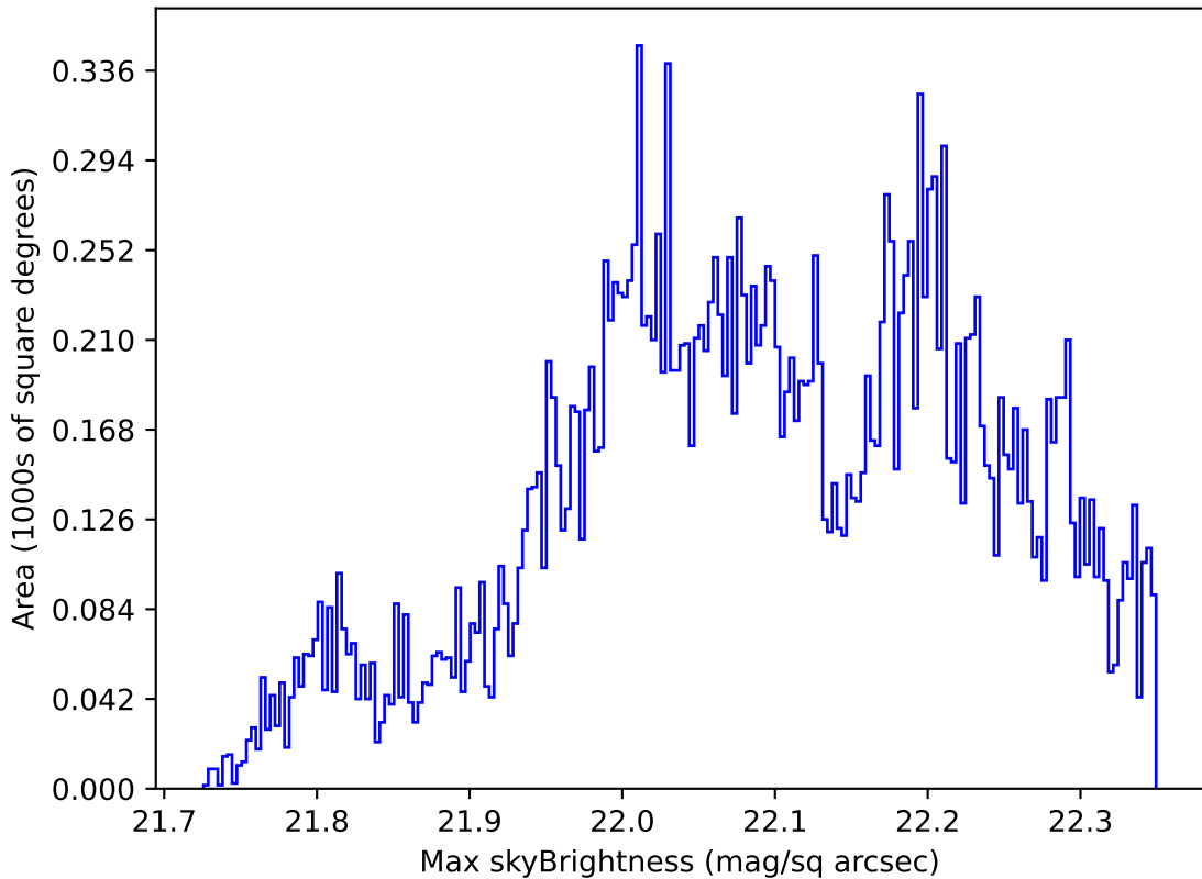
too_elab_r256_d2_ugrizy_v3.4_10yrs Yr 1 g band: Max skyBrightness
