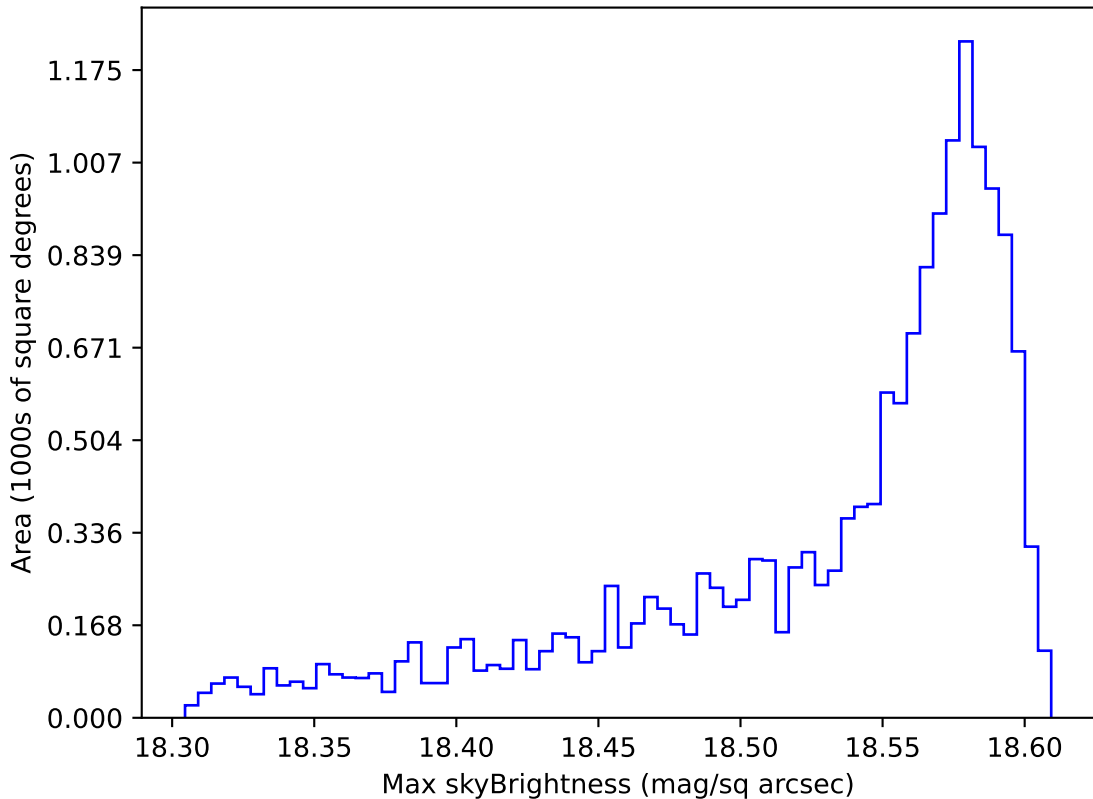
too_elab_r256_d2_ugrizy_v3.4_10yrs WFD y band: Max skyBrightness
