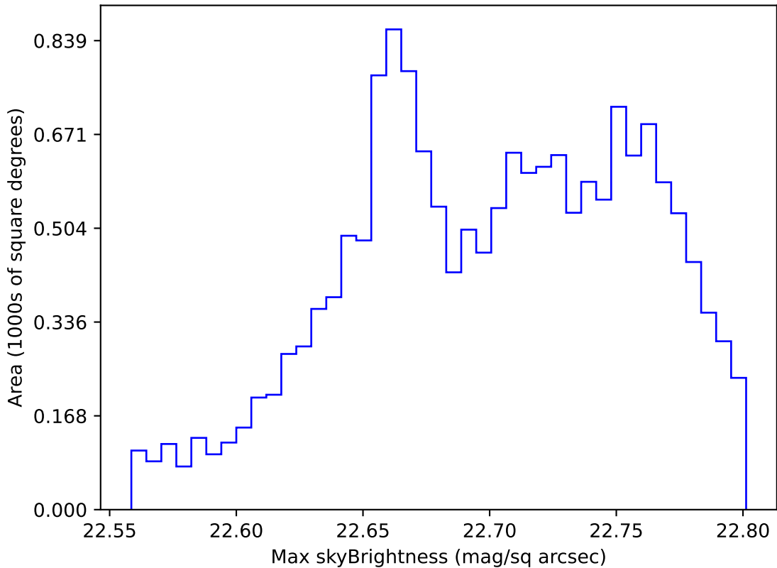
too_elab_r256_d2_ugrizy_v3.4_10yrs WFD u band: Max skyBrightness
