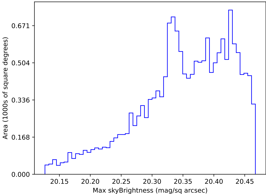
too_elab_r256_d2_ugrizy_v3.4_10yrs WFD i band: Max skyBrightness
