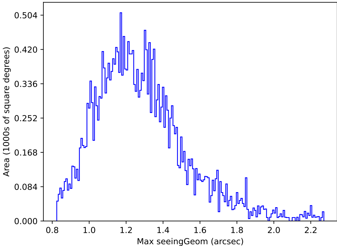
too_elab_r256_d2_ugrizy_v3.4_10yrs Yr 1 z band: Max seeingGeom
