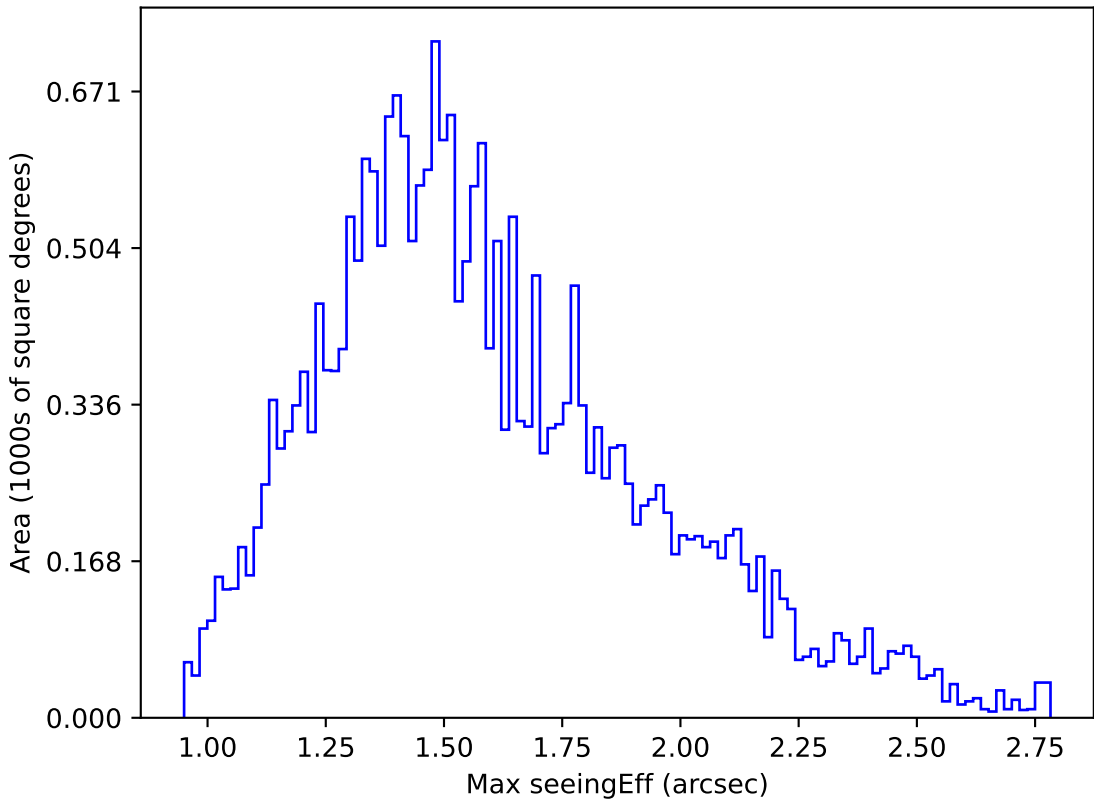
too_elab_r256_d2_ugrizy_v3.4_10yrs Yr 1 r band: Max seeingEff
