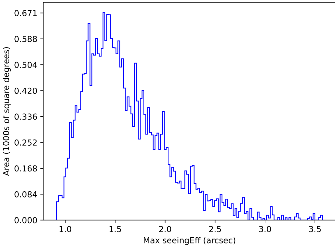
too_elab_r256_d2_ugrizy_v3.4_10yrs Yr 1 g band: Max seeingEff
