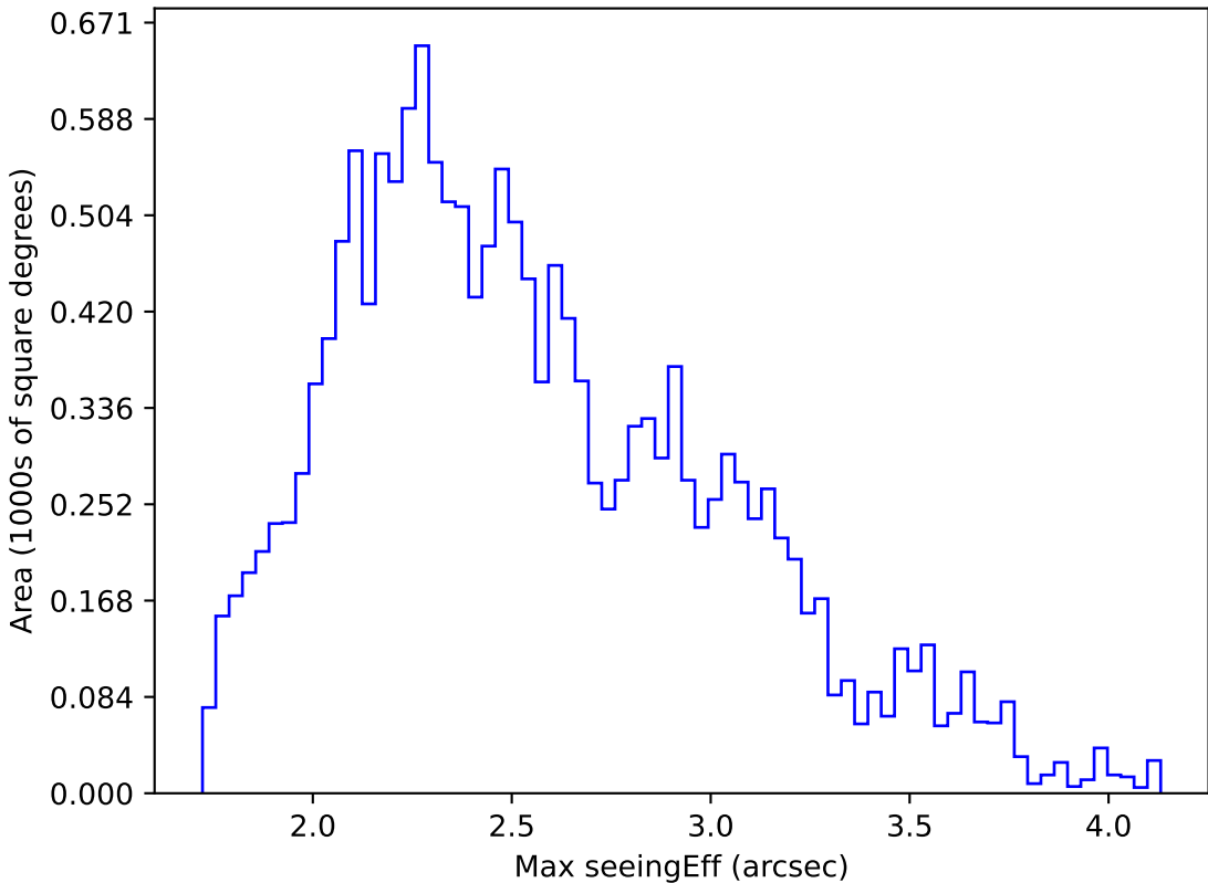
too_elab_r256_d2_ugrizy_v3.4_10yrs WFD u band: Max seeingEff
