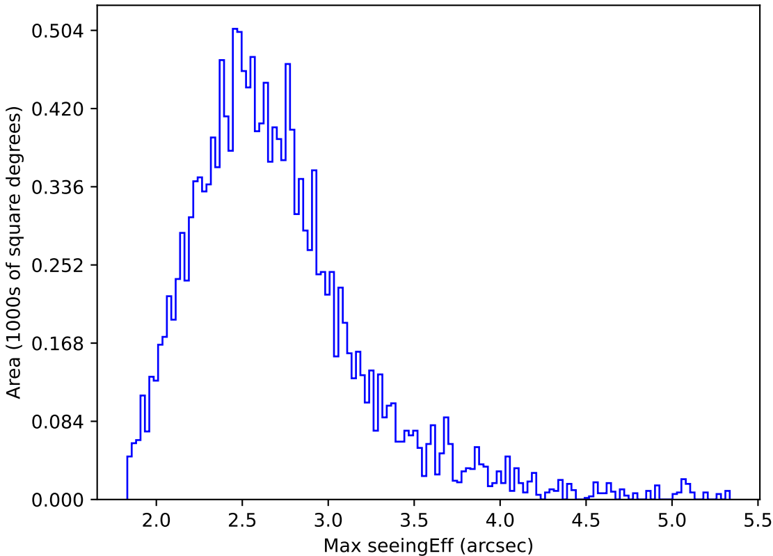
too_elab_r256_d2_ugrizy_v3.4_10yrs WFD r band: Max seeingEff
