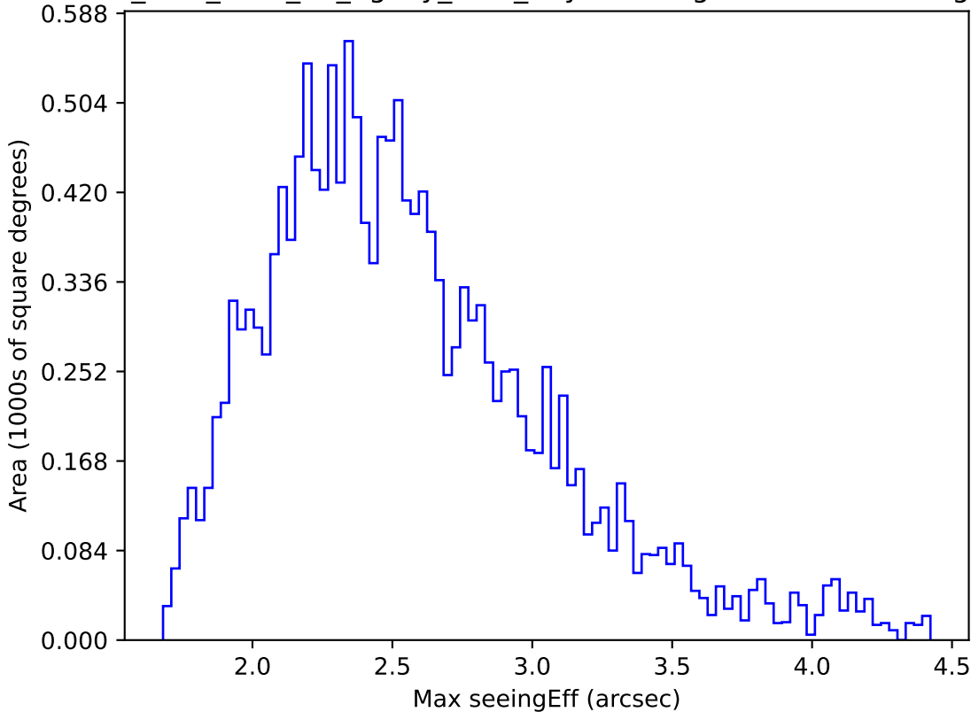
too_elab_r256_d2_ugrizy_v3.4_10yrs WFD g band: Max seeingEff
