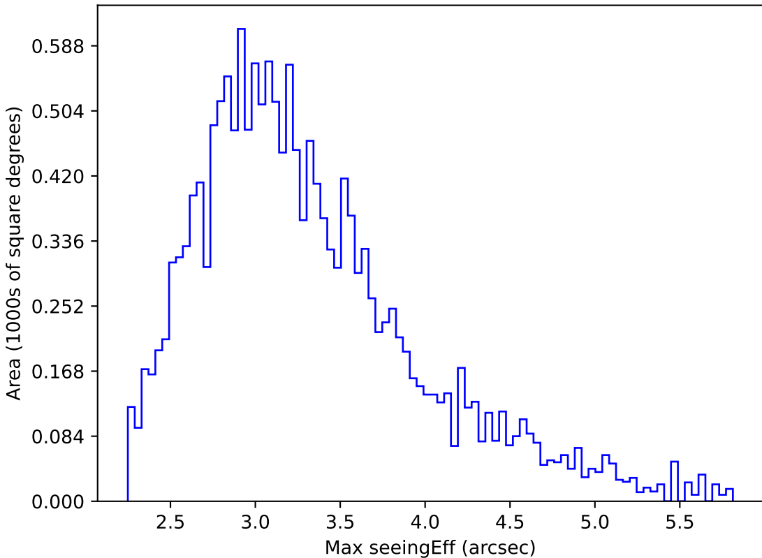
too_elab_r256_d2_ugrizy_v3.4_10yrs WFD all bands: Max seeingEff
