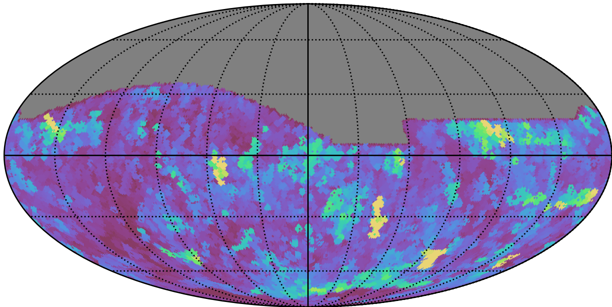
too_elab_r256_d2_ugrizy_v3.4_10yrs All sky z band: Max seeingEff
