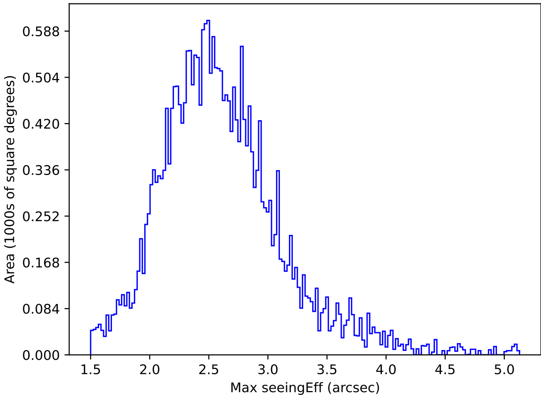
too_elab_r256_d2_ugrizy_v3.4_10yrs All sky r band: Max seeingEff
