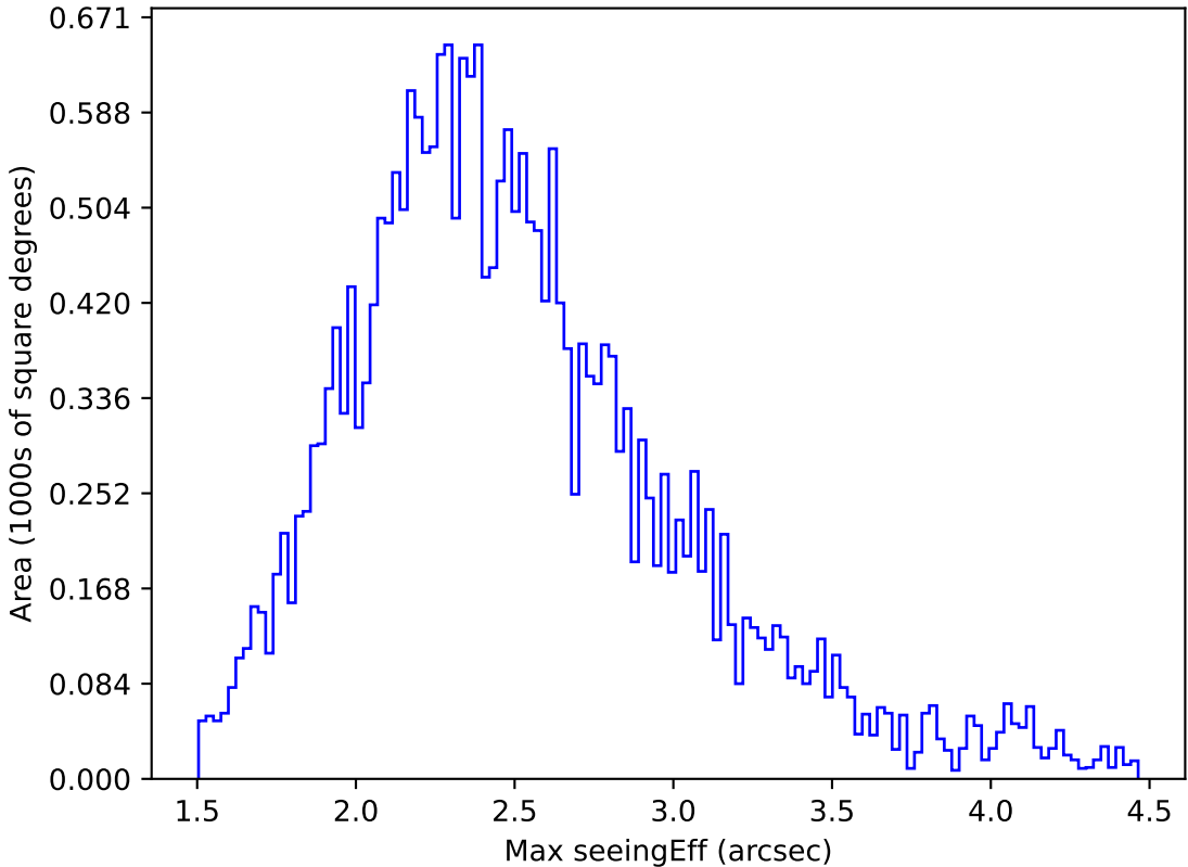
too_elab_r256_d2_ugrizy_v3.4_10yrs All sky g band: Max seeingEff
