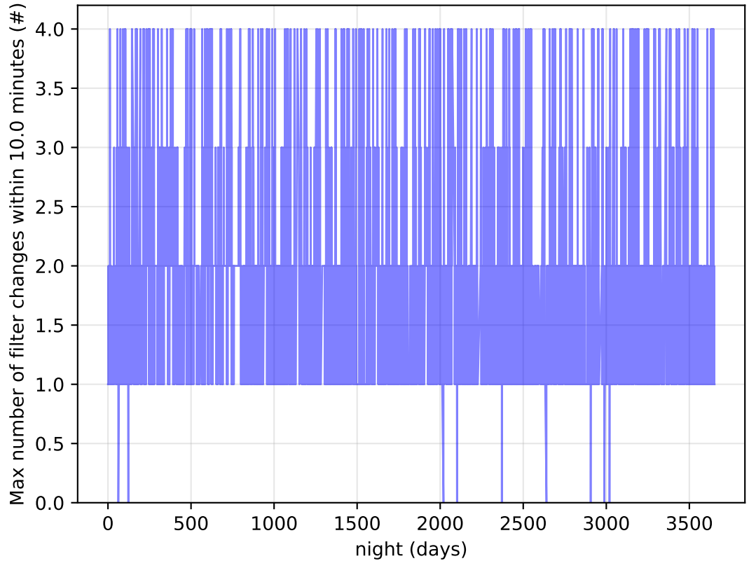
too_elab_r256_d2_ugrizy_v3.4_10yrs Per Night: Max number of filter changes within 10.0 minutes
