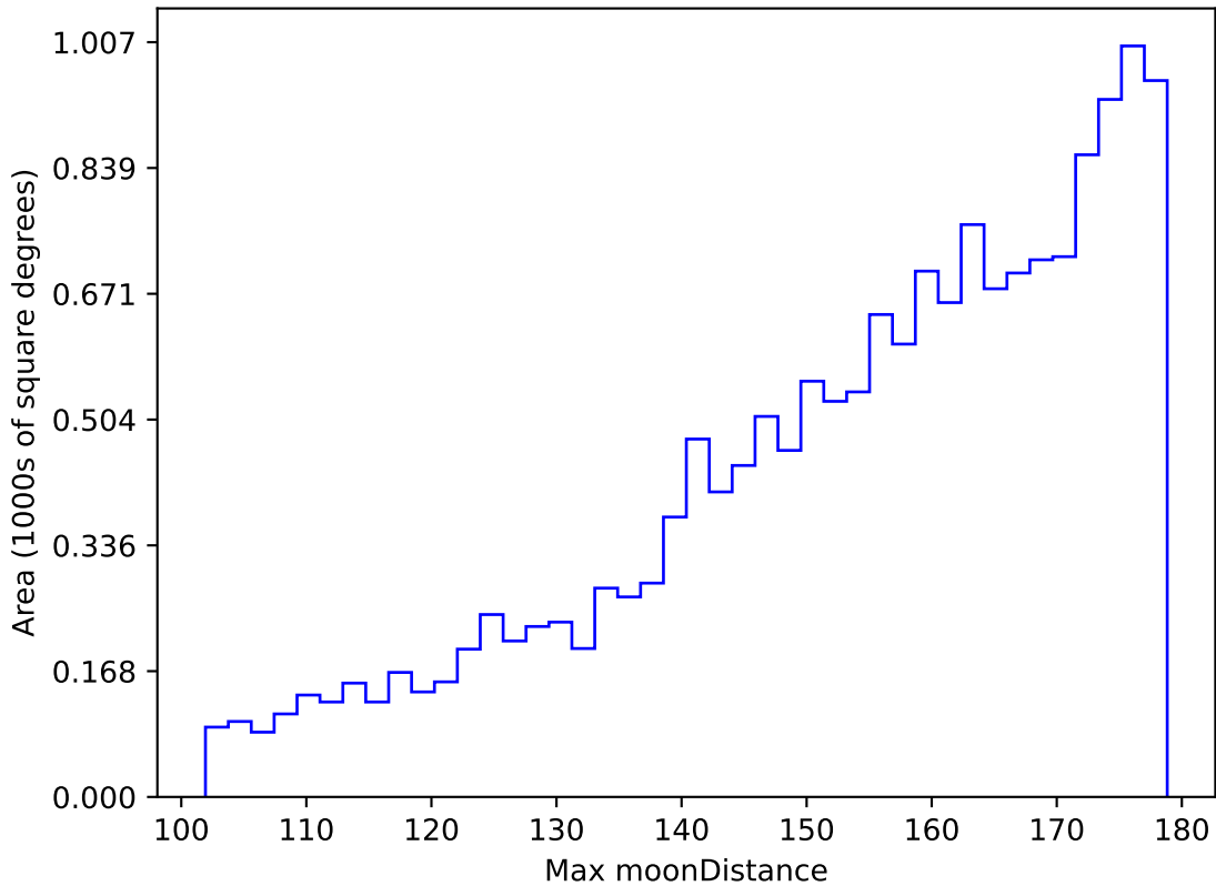
too_elab_r256_d2_ugrizy_v3.4_10yrs WFD u band: Max moonDistance
