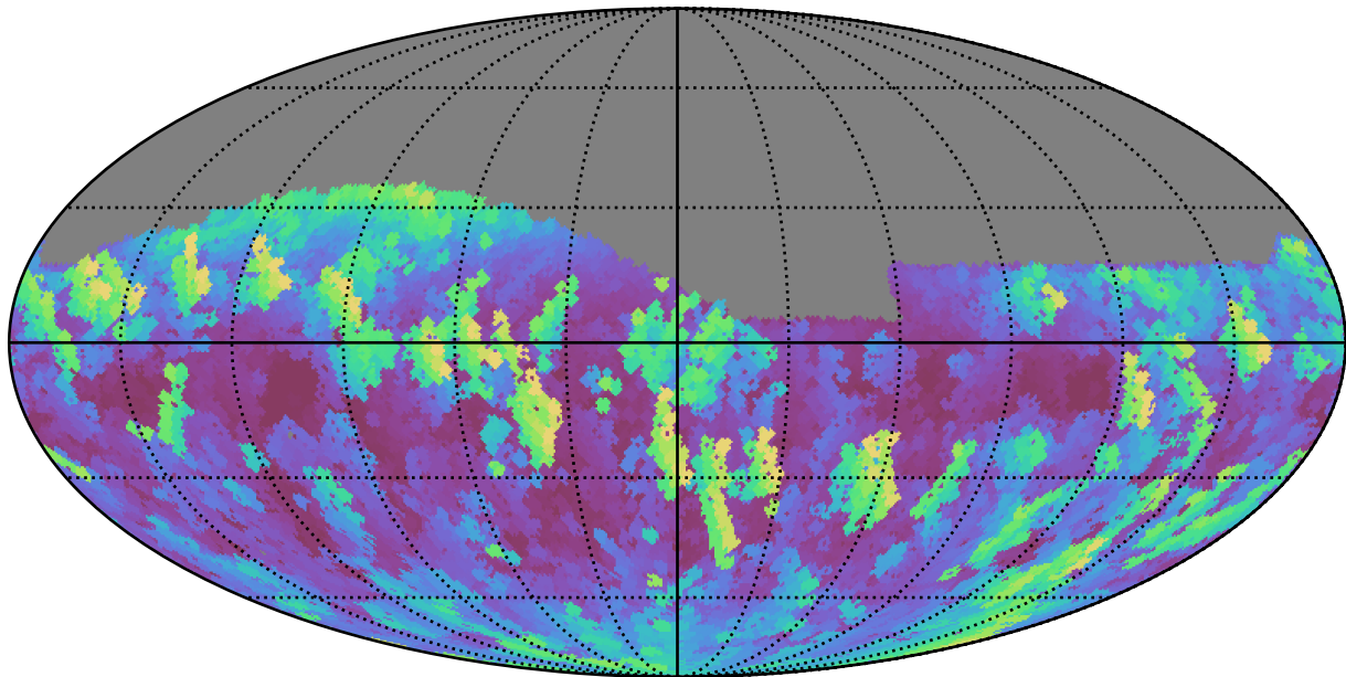
too_elab_r256_d2_ugrizy_v3.4_10yrs Yr 1 z band: Max airmass
