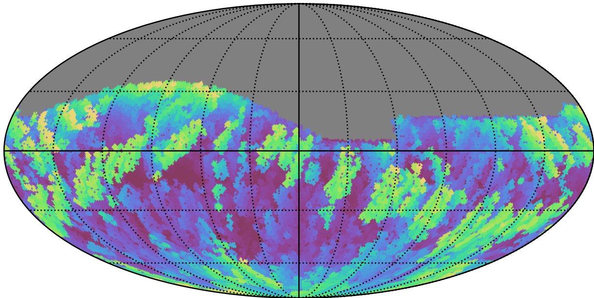
too_elab_r256_d2_ugrizy_v3.4_10yrs Yr 1 r band: Max airmass
