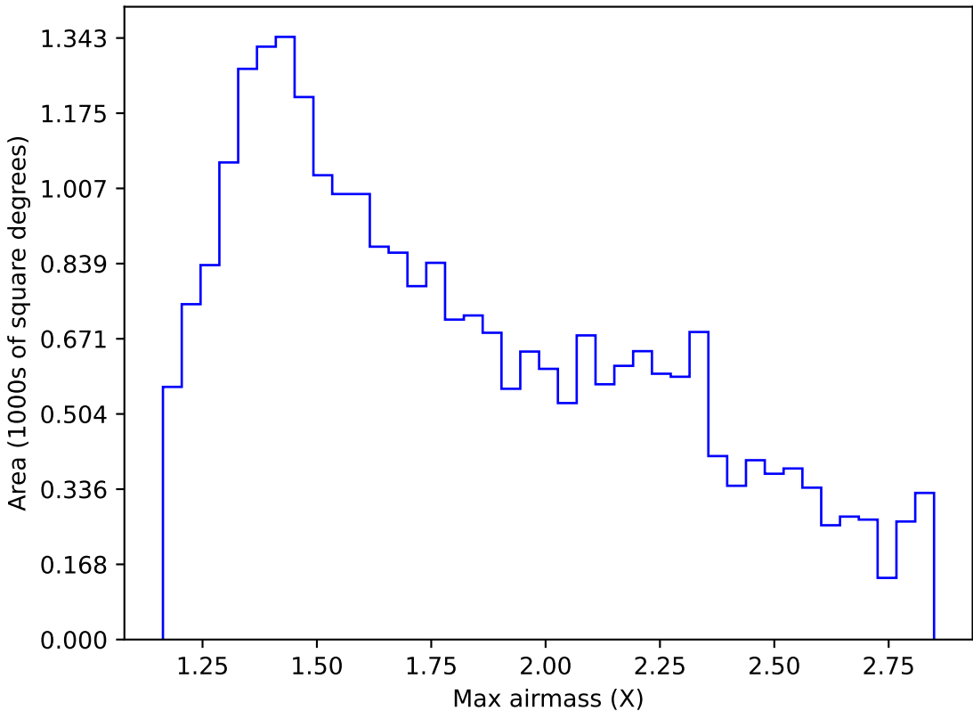
too_elab_r256_d2_ugrizy_v3.4_10yrs Yr 1 i band: Max airmass
