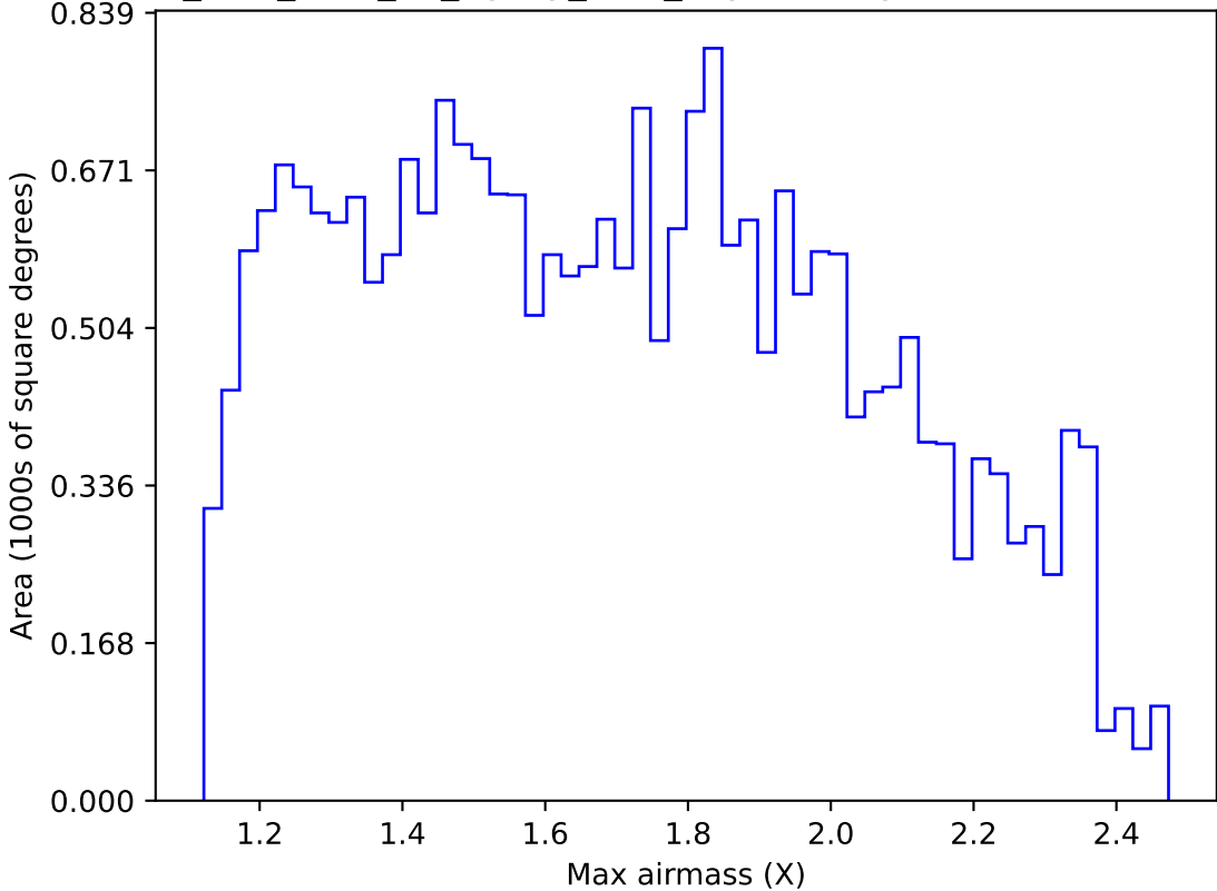
too_elab_r256_d2_ugrizy_v3.4_10yrs Yr 1 g band: Max airmass
