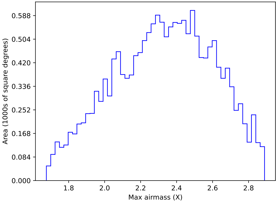
too_elab_r256_d2_ugrizy_v3.4_10yrs WFD y band: Max airmass
