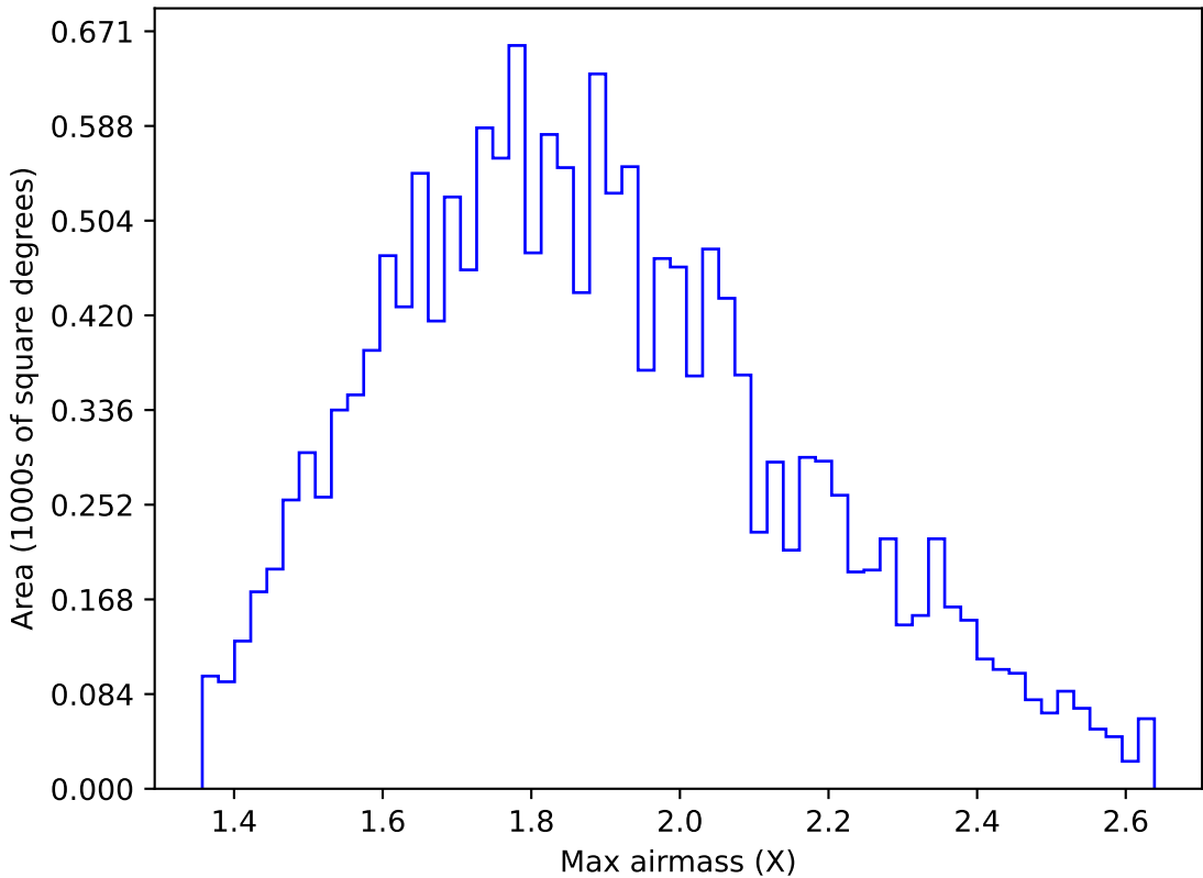
too_elab_r256_d2_ugrizy_v3.4_10yrs WFD u band: Max airmass
