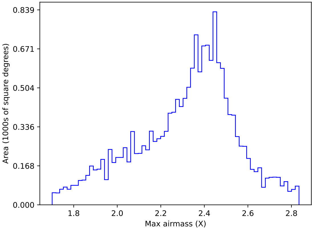
too_elab_r256_d2_ugrizy_v3.4_10yrs WFD r band: Max airmass
