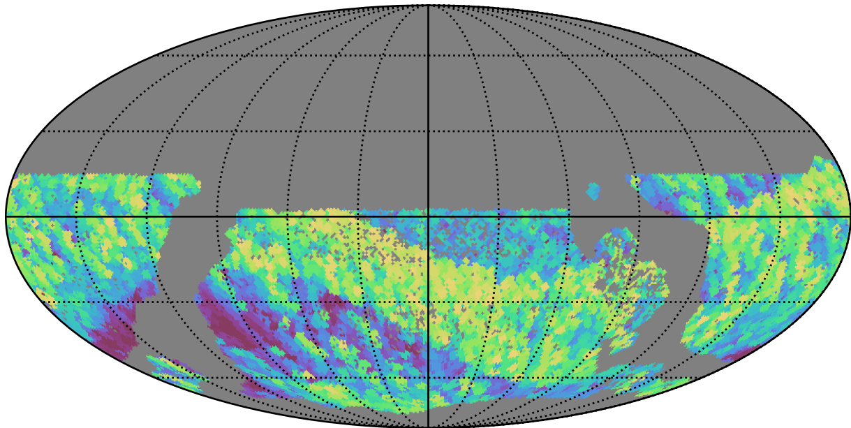
too_elab_r256_d2_ugrizy_v3.4_10yrs WFD i band: Max airmass
