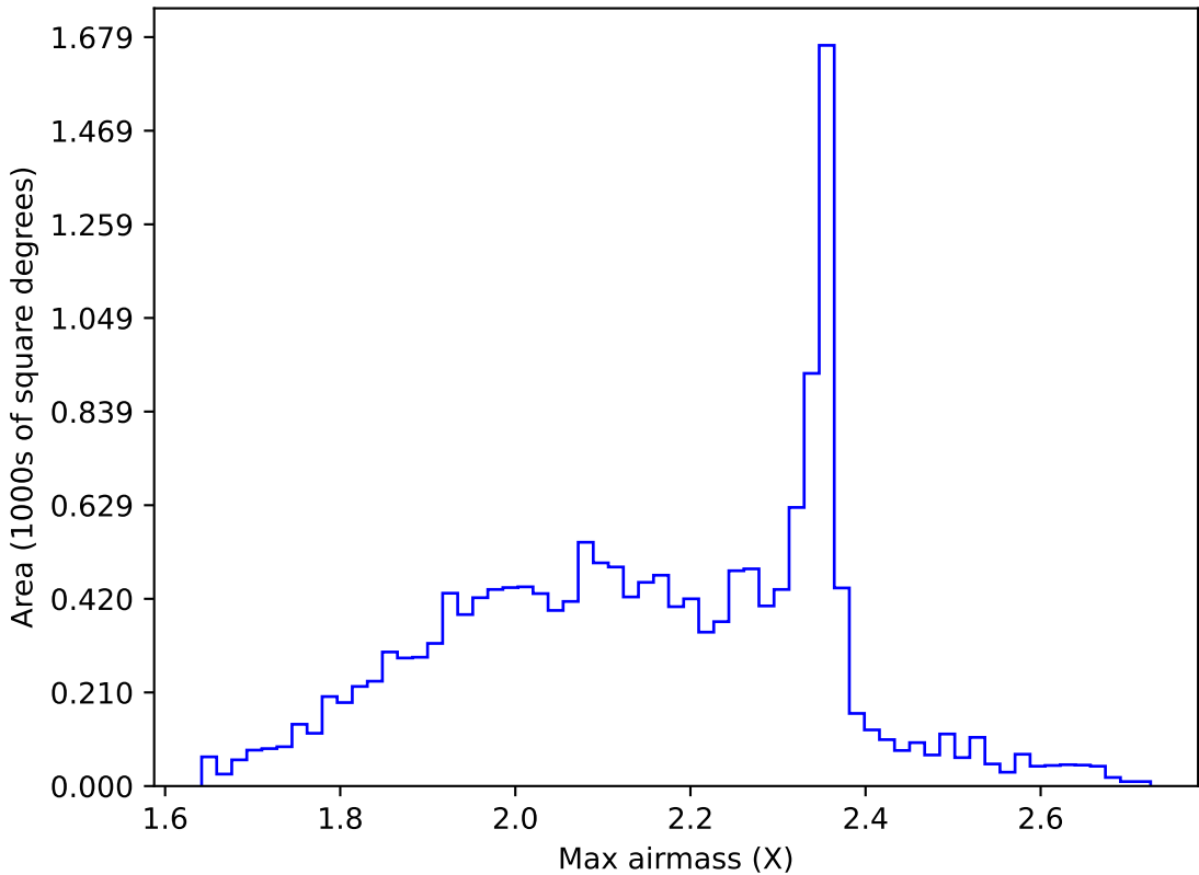
too_elab_r256_d2_ugrizy_v3.4_10yrs WFD g band: Max airmass
