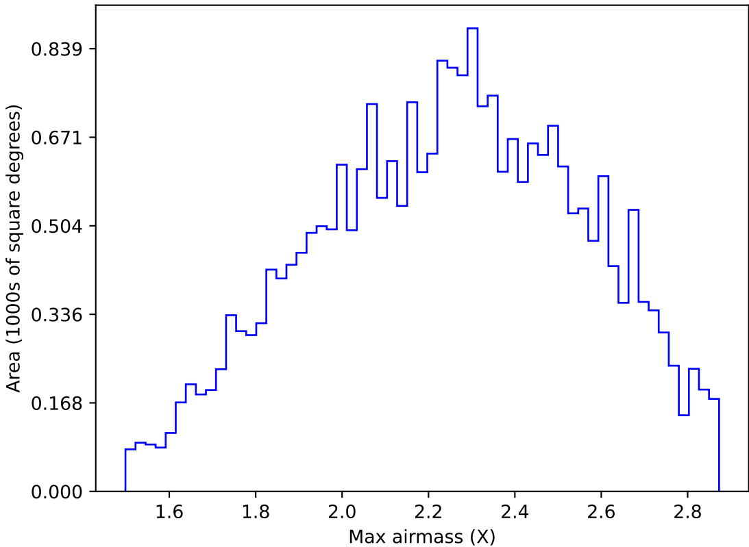
too_elab_r256_d2_ugrizy_v3.4_10yrs All sky y band: Max airmass
