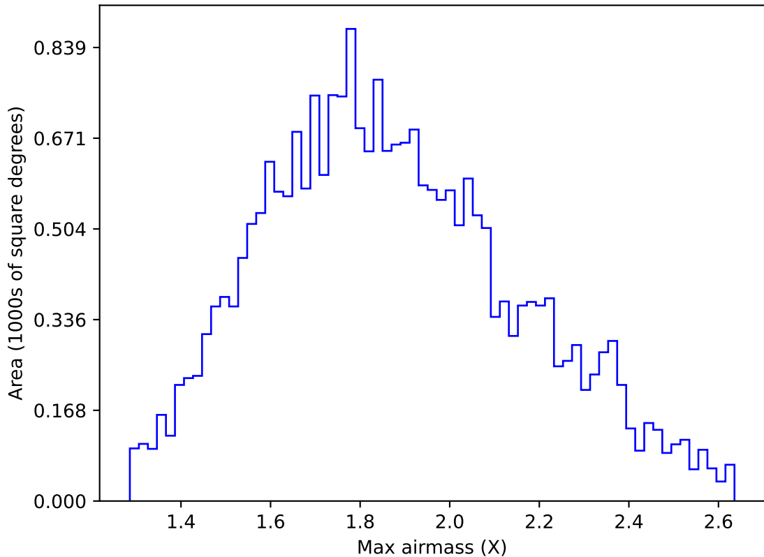
too_elab_r256_d2_ugrizy_v3.4_10yrs All sky u band: Max airmass
