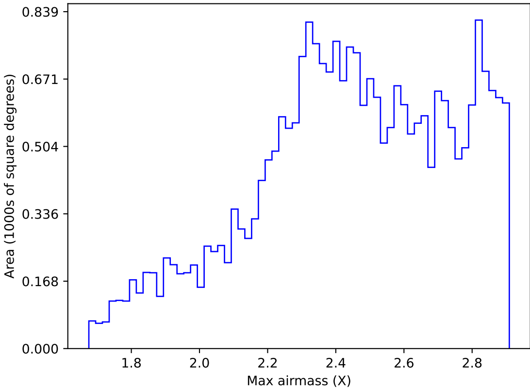
too_elab_r256_d2_ugrizy_v3.4_10yrs All sky i band: Max airmass
