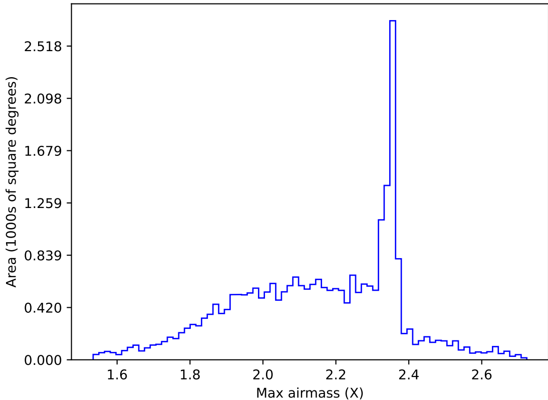
too_elab_r256_d2_ugrizy_v3.4_10yrs All sky g band: Max airmass
