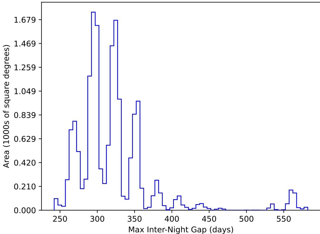
too_elab_r256_d2_ugrizy_v3.4_10yrs WFD y band: Max Inter-Night Gap
