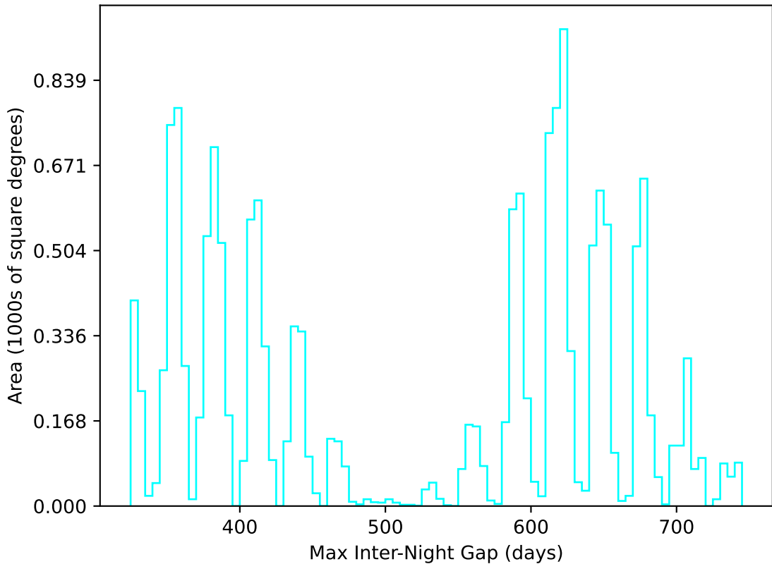
too_elab_r256_d2_ugrizy_v3.4_10yrs WFD u band: Max Inter-Night Gap
