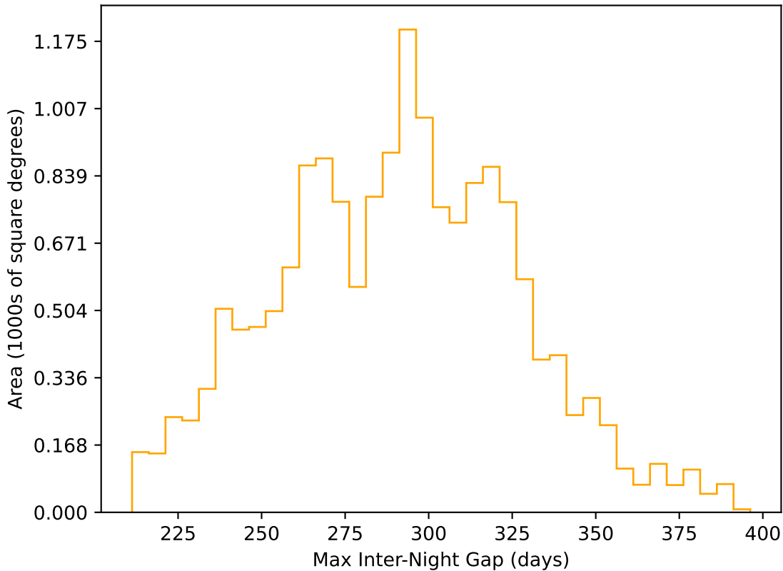
too_elab_r256_d2_ugrizy_v3.4_10yrs WFD r band: Max Inter-Night Gap
