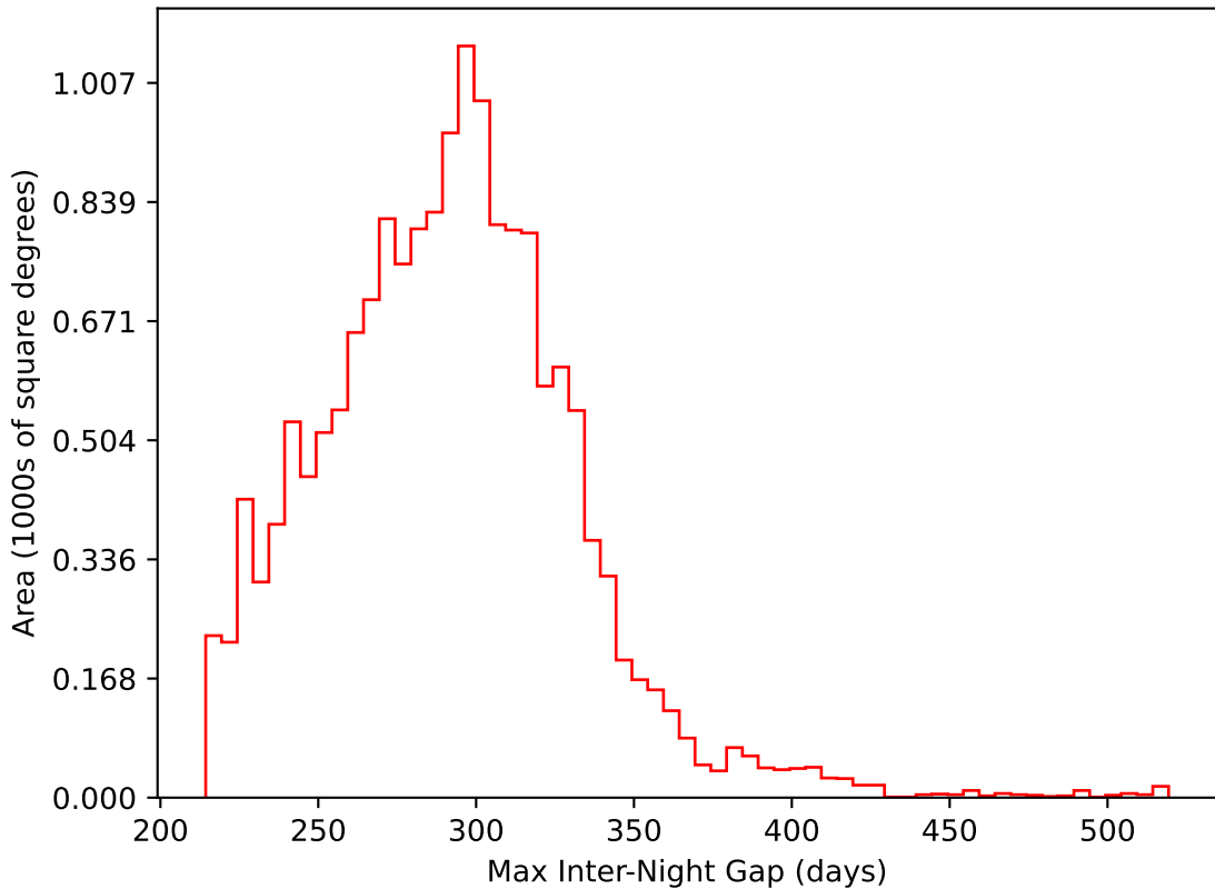
too_elab_r256_d2_ugrizy_v3.4_10yrs WFD i band: Max Inter-Night Gap
